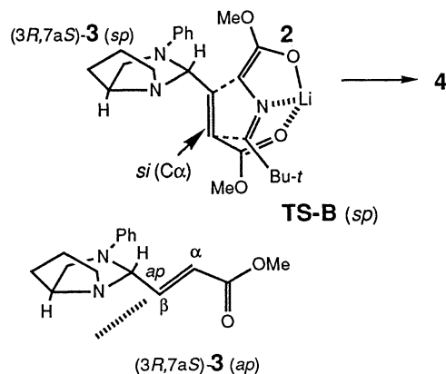
Fig. 1. Proposed transition state for the asymmetric Michael addition of N -lithiated azomethine ylide 2 to (3R,7aS)\text{-}3 .
